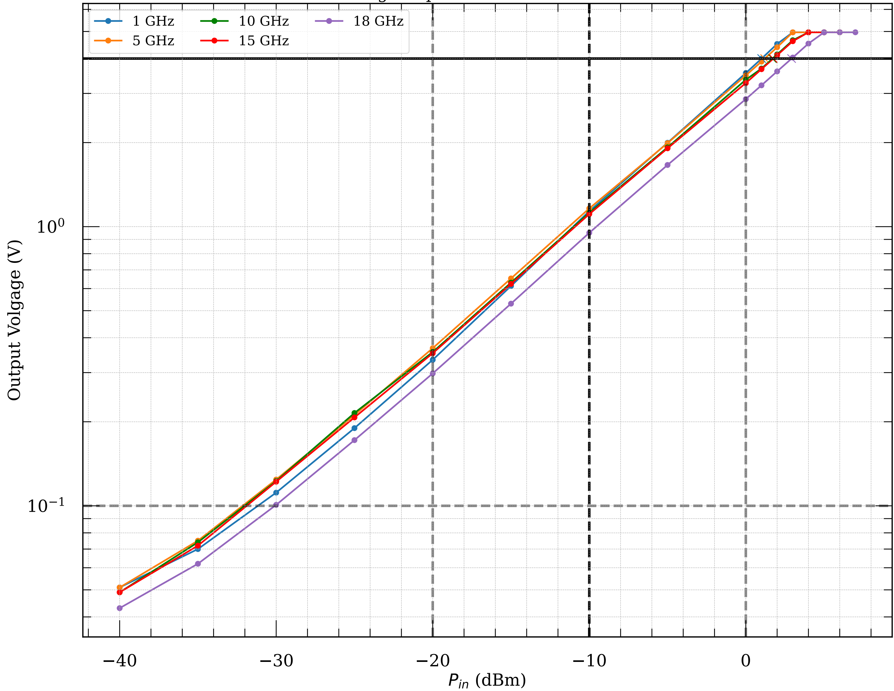
Measured voltage-to-power curve of detector module096
